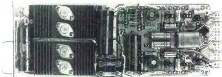
Solid-state AA-601 Audio Distribution Module provides 6 outputs at \pm 24 dbm \sim 600 ohms balanced, or other combinations, as required. Modules can be added to system as requirements grow.
