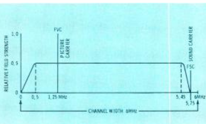
Fig. 2b Vestigial sideband transmission. Picture carrier has been moved to the left of center—the lower channel edge. Lower sideband has been suppressed. This permits 4.5 MHz of video modulation.
