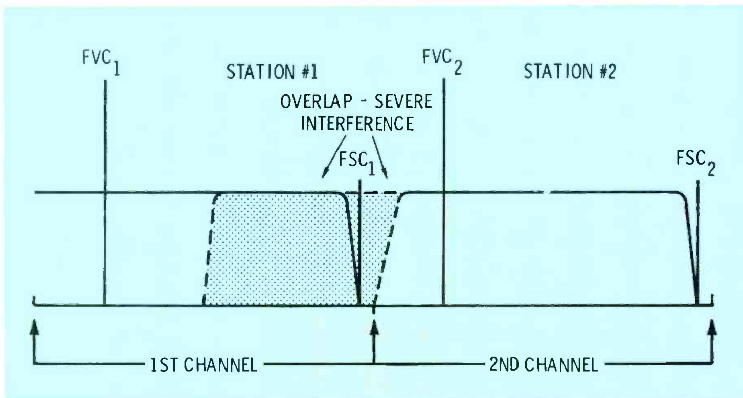
Fig. 3 Severe interference would be caused if the lower sideband were allowed to overlap the adjacent channel. The amount of overlap is shown in the shaded area.
