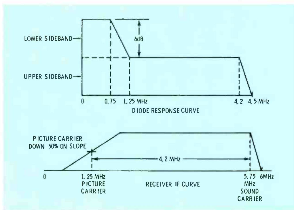
Fig. 4a Diode response curve.
