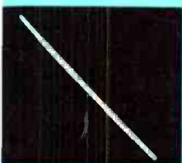
Fig. 5 Waveforms produced by resistance, capacitance or inductance without a transistor. (A) A 3.3K-ohm resistor across the test leads gives this tilted waveform. (B) Either a .47 mfd capacitor or a filter choke across the test leads produces a near-circle.
