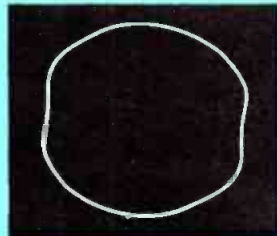
Fig. 5 Waveforms produced by resistance, capacitance or inductance without a transistor. (A) A 3.3K-ohm resistor across the test leads gives this tilted waveform. (B) Either a .47 mfd capacitor or a filter choke across the test leads produces a near-circle.
