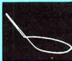
(D) A PNP germanium transistor with the emitter connected to G, the base to H through a 6.8K-ohm resistor, and a 6.8K resistor in parallel with the base and emitter. The waveform approaches that of a pure resistance, but the diode corner is still visible.
